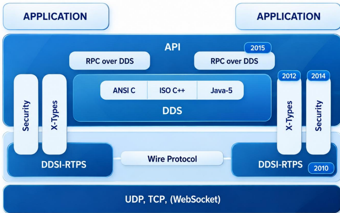
Figure 3 – OMG DDS Architecture
