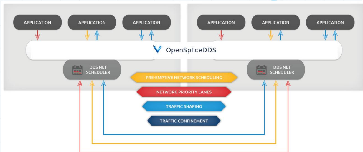
Figure 2: OpenSpliceDDS Network Scheduler and its Network priority Lanes
