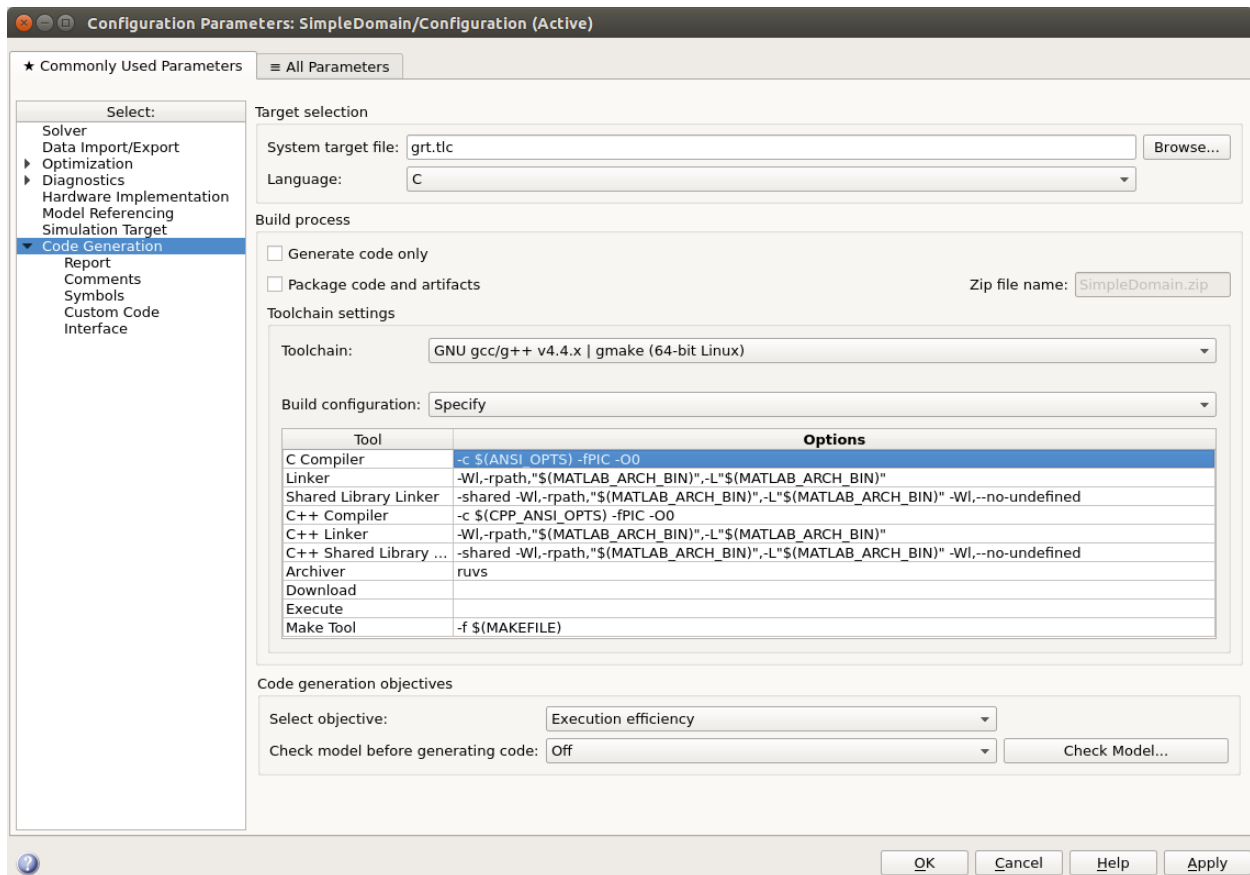
Fig. 1: C/C++ Code Generation Options. Remove the text $(ANSI_OPTS) for C Compiler to avoid compile errors.
